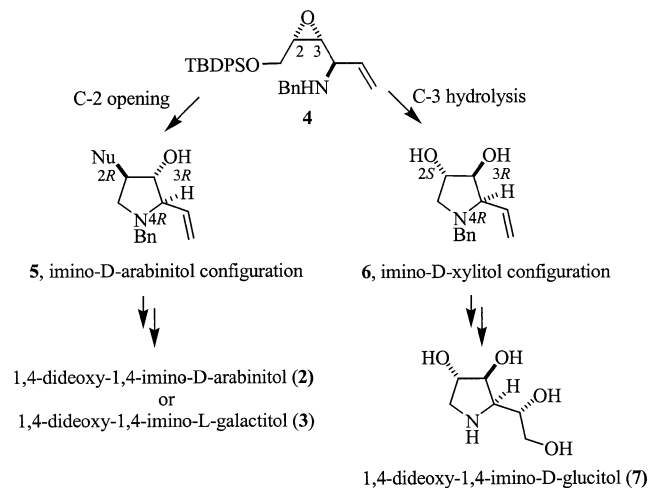
Scheme 1. Stereocontrolled access to five-membered ring imino sugars from the versatile epoxyamine 4
