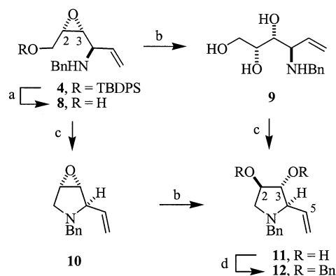
Scheme 2. a: TBAF supported on silica gel, THF, room temp., 87%; b: 3 M H 2 SO 4 / p -dioxane, reflux, 70% of 9 from 8 , 85% of a 94:6 mixture of 11 and its diastereomer from 10 ; c: Ph 3 P, CCl 4 , Et 3 N, DMF, room temp., 71% of 10 from 8 , 67% of 11 from 9 ; d: NaH, BnBr, Bu 4 NI, THF, 80%
