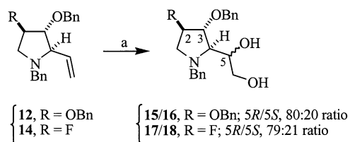
Scheme 4. a: OsO 4 , NMO, p -dioxane/H 2 O, 70 °C, 69% of a 80:20 mixture of 15 and 16 from 12 , 80% of a 79:21 mixture of 17 and 18 from 14
