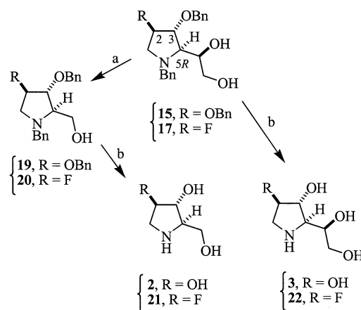
Scheme 5. a: NaIO 4 then NaBH 4 , EtOH/H 2 O, room temp., 70% of 19 from 15 , 70% of 20 from 17 ; b: Pd/C, 10 bar H 2 , cat. 12 M HCl, MeOH, 94–98%
