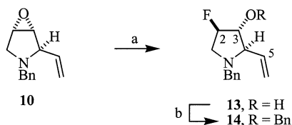
Scheme 3. a: HF·pyridine, 60 °C, 85% of a 92:8 mixture of 13 and its regioisomer; b: NaH, BnBr, Bu 4 NI, THF, 83%
